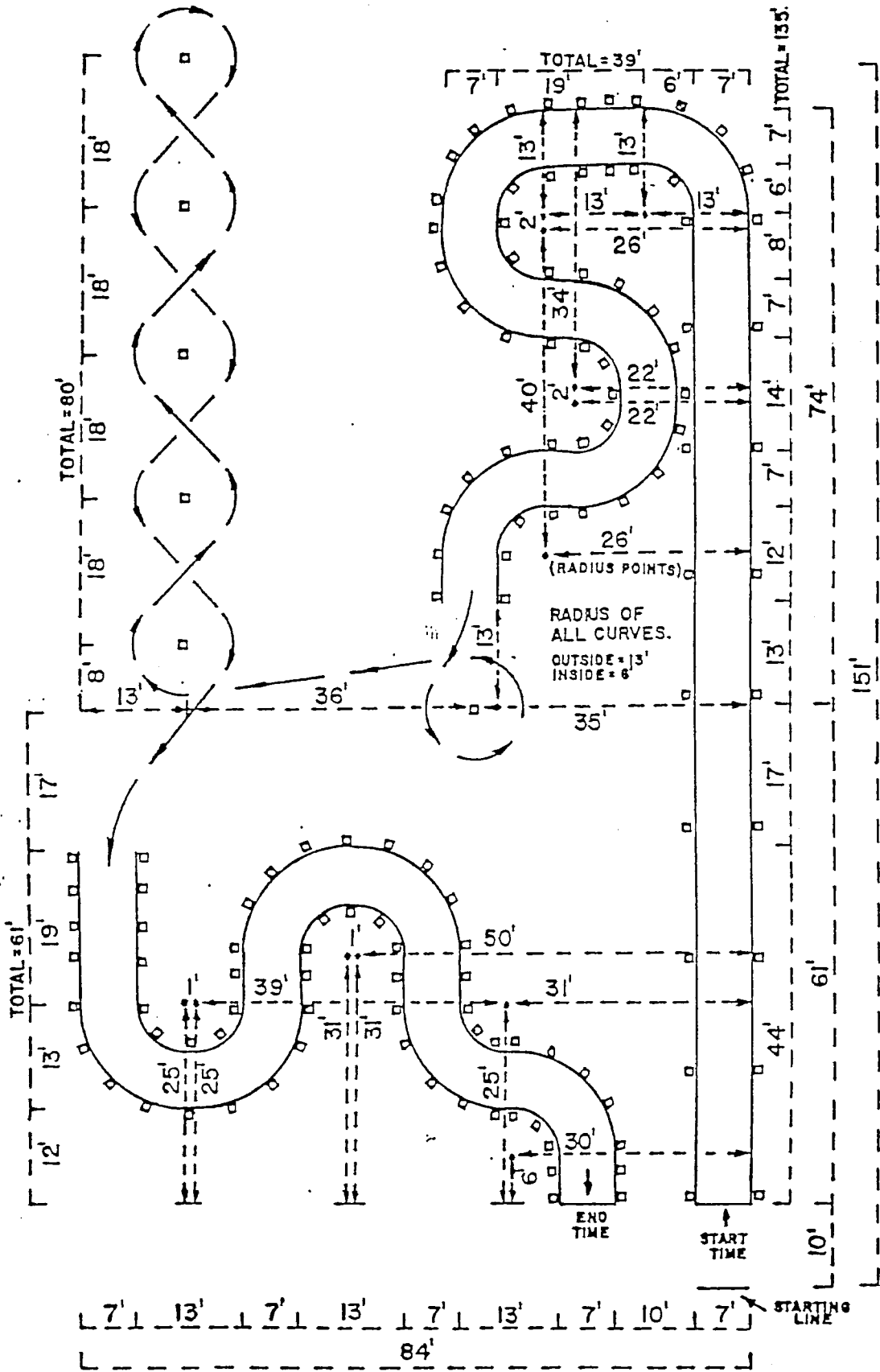
TEXAS SHRINE MOTOR PATROL ASSOCIATION OBSTACLE COURSE (NOT TO SCALE)
